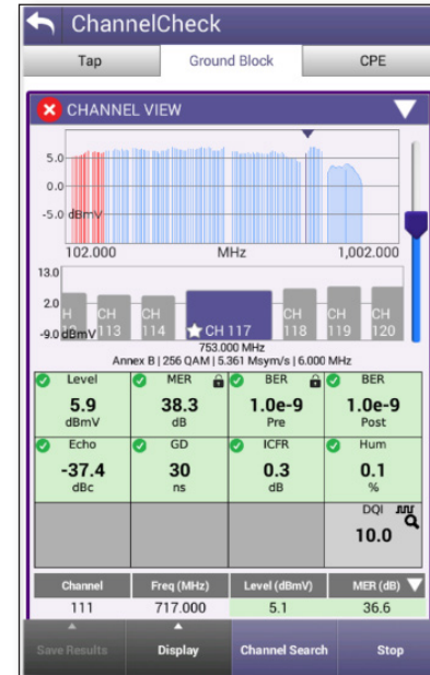
ONX-620 – Level & MER measurement
