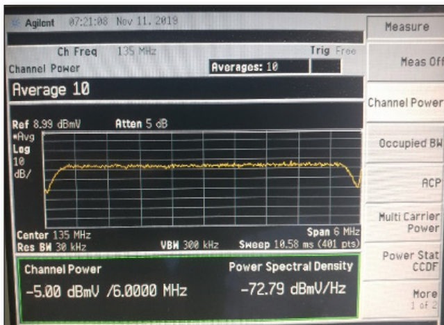
Agilent E4402B Spectrum Analyzer – Channel power measurement
