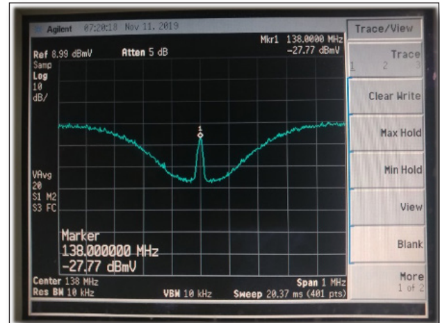
Agilent E4402B SA – Tag level measurement
